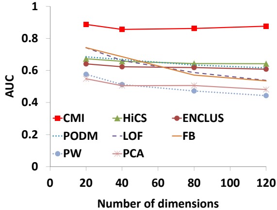
(b) AUC vs. dimensionality
