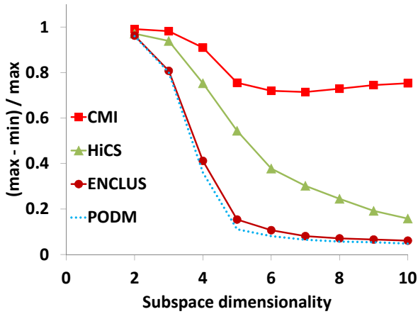
(a) Contrast score vs. dimensionality
