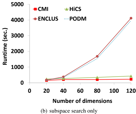
Figure 3: Runtime w.r.t. dimensionality
